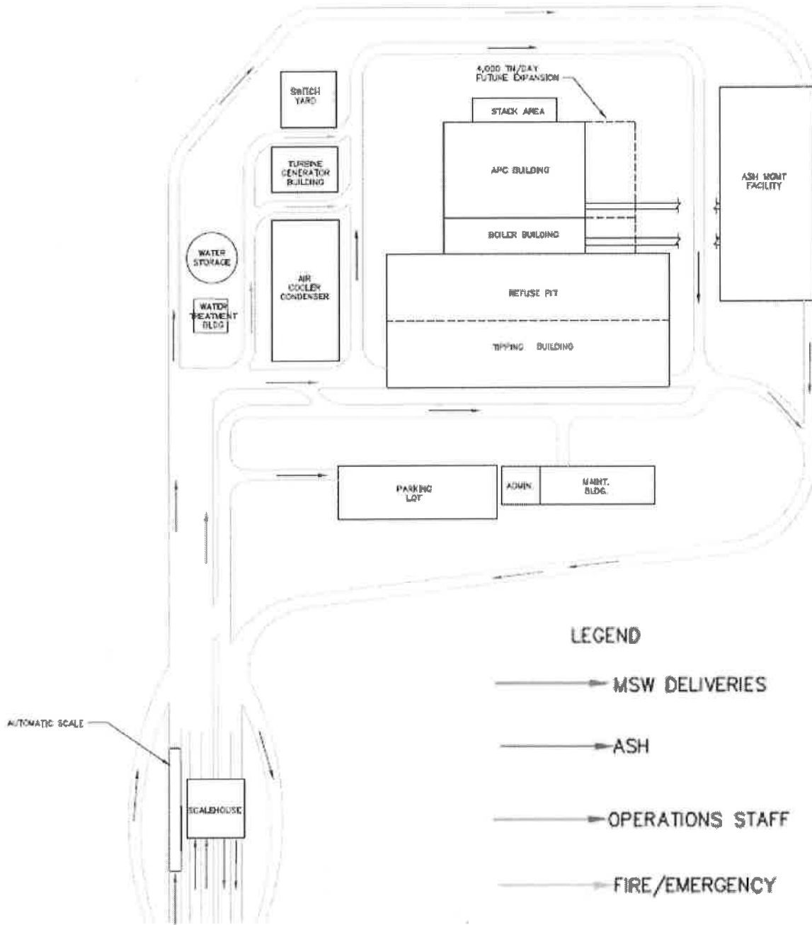
Figure 3-2. Conceptual Layout for Layout Option 1 (Low Bound Forecast)
